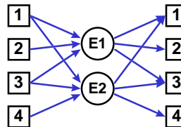
Tripartite representation
