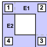
Connection hypergraph
