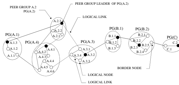
Figure 5: ATM-network
